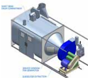
ISOMETRIC VIEW INTERNAL CONTAINER WITH FAN SYSTEM NOT EXTRACTED
