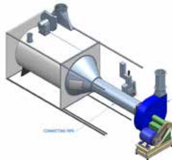
ISOMETRIC VIEW INTERNAL CONTAINER WITH FAN SYSTEM EXTRACTED
