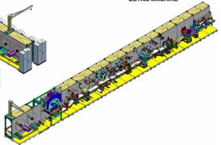
ISOMETRIC VIEW BOTTOM DETAIL MACHINE
