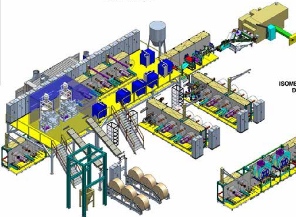
ISOMETRIC VIEW
